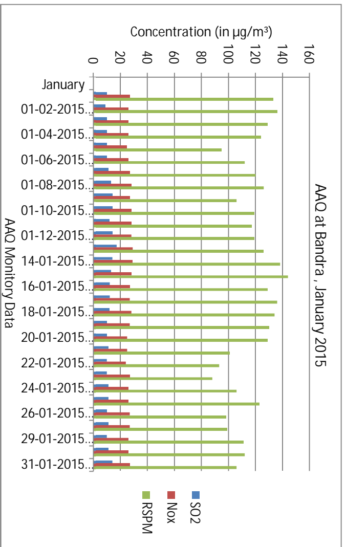
Figure 3.42 AAO at Bandra, January 2015
